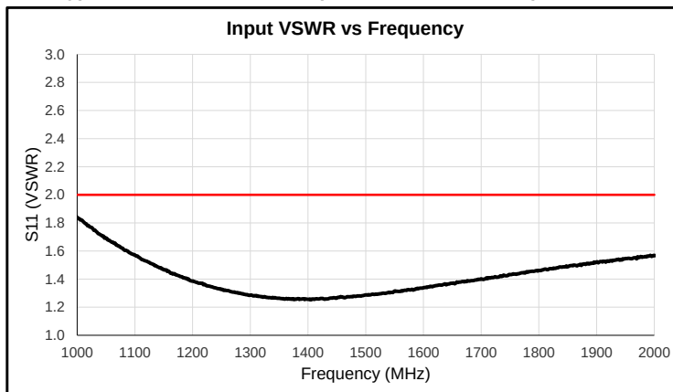
Typical Performance @ 23°C (Reference S/N 2137904)
